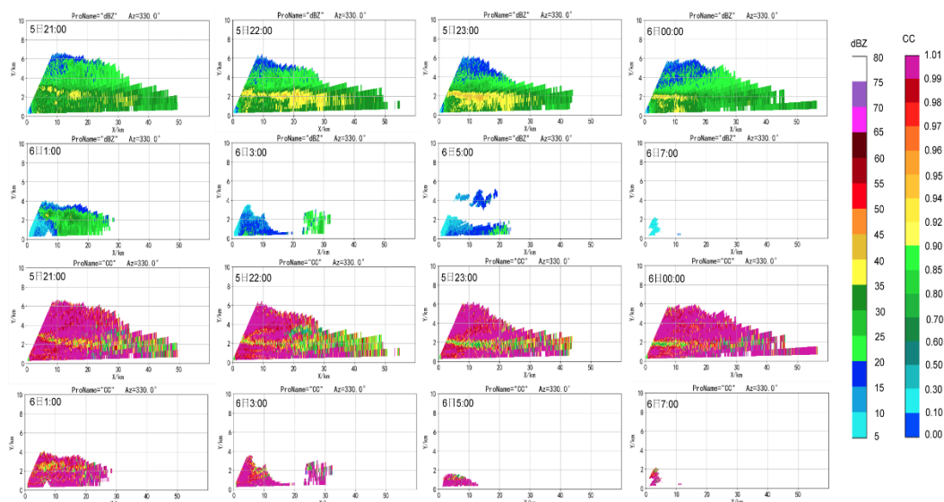
Fig. 10 (a) Reflectivity factor and (b) correlation coefficient at Sujiatun X-band dual-polarization phased array radar at 6.3 °elevation from 21:00 BT 5 to 07:00 BT 6 November 2023
