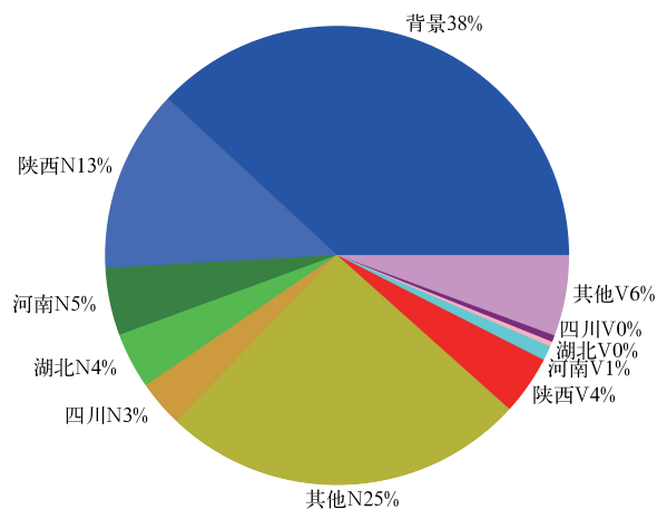
图 6 2023 年暖季陕西 O_3 来源解析 Fig. 6 Apportionment of O_3 sources in Shaanxi Province in the warm season of 2023
