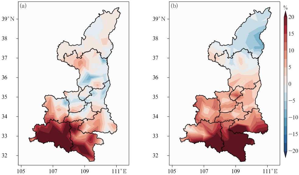
图 3 (a)2020 年和(b)2022 年暖季陕西 O 3 气象条件评估指数较上一年同期变化率的空间分布 Fig. 3 Spatial distribution of changes in O 3 meteorological condition evaluation index in Shaanxi Province in the warm season of (a) 2020 and (b) 2022 compared to that in the same period of the previous year
