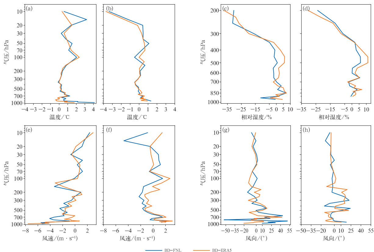
图 4 2023 年 8 月 31 日 00 时至 9 月 6 日 00 时(a, c, e, g)00 时和(b, d, f, h)12 时北斗探空下降段与 FNL 分析场和 ERA5 再分析资料的(a, b)温度, (c, d)相对湿度, (e, f)风速, (g, h)风向平均偏差 Fig. 4 The average deviations of (a, b) temperature, (c, d) relative humidity, (e, f) wind speed, and (g, h) wind direction from FNL analysis field and ERA5 reanalysis data during the descending segment of Beidou sounding at (a, c, e, g) 00:00 UTC and (b, d, f, h) 12:00 UTC from 00:00 UTC 31 August to 00:00 UTC 6 September 2023
