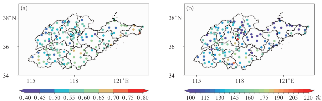
图 4 1966—2023 年山东强降水(a)降水量与降水持续时长的 Kendall 秩相关系数和(b)降水次数的空间分布 Fig. 4 Spatial distribution of (a) Kendall correlation coefficients between precipitation amount and duration and (b) frequency of heavy precipitation in Shandong Province during 1966—2023
