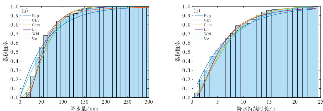
图 5 1966—2023 年崂山站强降水的 (a) 降水量和 (b) 降水持续时长的频率分布及候选边缘分布拟合 Fig. 5 Frequency distribution and candidate marginal distribution fitting of (a) precipitation amount and (b) duration of heavy precipitation at Laoshan Station during 1966–2023
