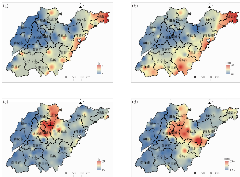
图 2 1966—2023 年山东强降水(a)平均持续时长,(b)平均降水量,(c)最长持续时长和(d)最大降水量 Fig. 2 (a) Mean duration, (b) mean precipitation amount, (c) the longest duration and (d) maximum precipitation amount of heavy precipitation in Shandong Province during 1966—2023
