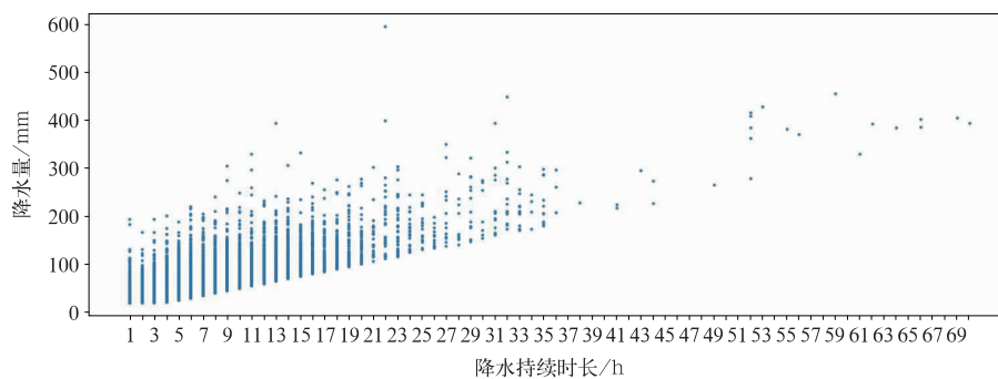
图 3 1966—2023 年山东强降水的降水量与降水持续时长散点分布 Fig. 3 Scattered distribution of precipitation amount and duration of heavy precipitation in Shandong Province during 1966—2023
