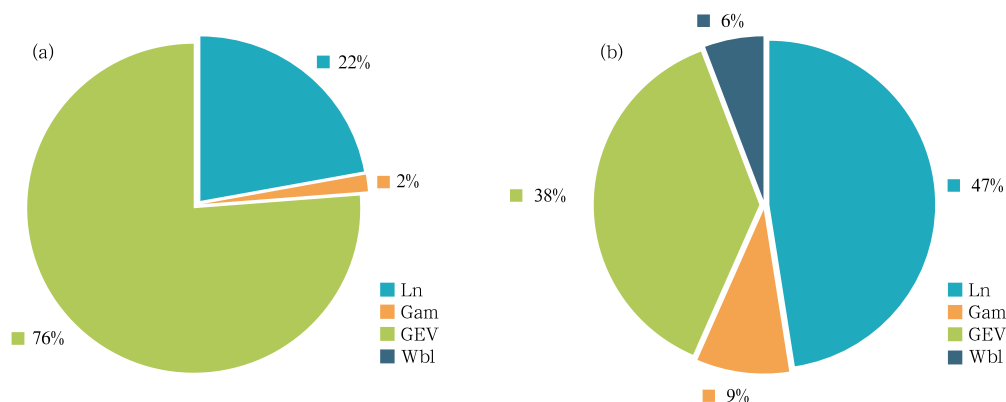
图 6 1966—2023 年山东 122 个观测站强降水的 (a) 降水量和 (b) 降水持续时长最优边缘分布占比 Fig. 6 Percentage of optimal marginal distribution of (a) precipitation amount and (b) duration of heavy precipitation at 122 stations in Shandong Province during 1966–2023
