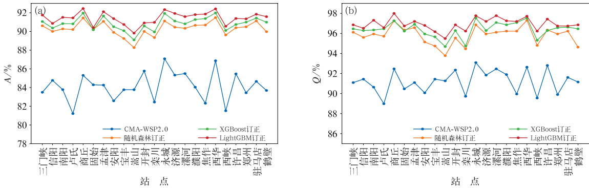
图 5 2022 年河南省各站点测试集中 CMA-WSP2.0 预报,随机森林、XGBoost、LightGBM 订正的总辐照度 24 h(a) A 、(b) Q Fig. 5 (a) A and (b) Q in 24 h of total irradiance predicted by CMA-WSP2.0 and corrected by random forest, XGBoost and LightGBM at each station in Henan Province in the test set in 2022
