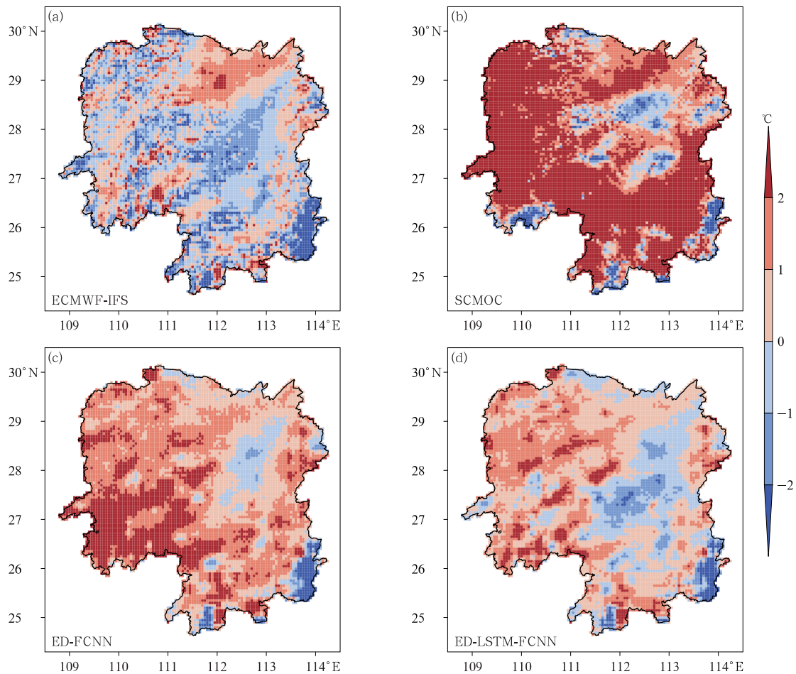
图 11 2022 年 11 月 29 日 11 时湖南不同预报产品气温预报值与观测值偏差的空间分布 Fig. 11 Spatial distribution of the deviation between different temperature forecast products and observations in Hunan Province at 11:00 BT 29 November 2022
