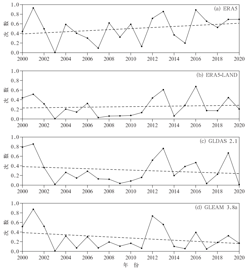
图 5 (a)ERA5,(b)ERA5-LAND,(c)GLDAS 2.1 和 (d)GLEAM 3.8a 资料中淮河流域 2000—2020 年逐年骤旱发生次数 Fig. 5 Annual occurrence count of flash droughts in the Huaihe River Basin in (a) ERA5, (b) ERA5-LAND, (c) GLDAS 2.1 and (d) GLEAM 3.8a datasets from 2000 to 2020
