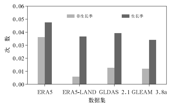
图 6 淮河流域 2000—2020 年骤旱在作物 非生长季和生长季的区域月平均发生次数 Fig. 6 Regional monthly average occurrence count of flash droughts in the Huaihe River Basin during non-growing and growing seasons of crops from 2000 to 2020
