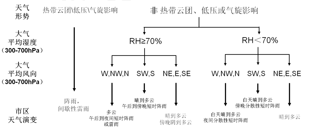
338 图 9 2023 年太平洋运动会现场气象保障专家组归纳的霍尼亚拉市天气预报决策流程图 339 Fig. 9 Decision flowchart of weather forecast summarized by the on-site meteorological support expert group for 340 Honiara City of Pacific Games in 2023
