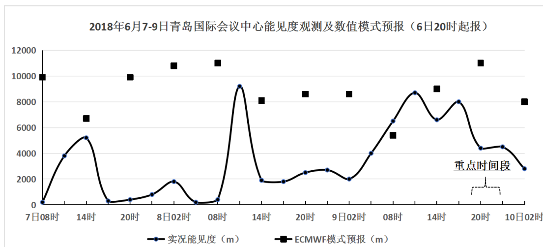
图 4 2018 年 6 月 7—9 日青岛国际会议中心能见度观测及 EC 模式 6 日 20: 00 起报的能见度预报 Fig.4 Visibility observation and the forecast initiated at 20:00 BT 6 by EC model at the Qingdao International Conference Center from 7 to 9 June 2018
