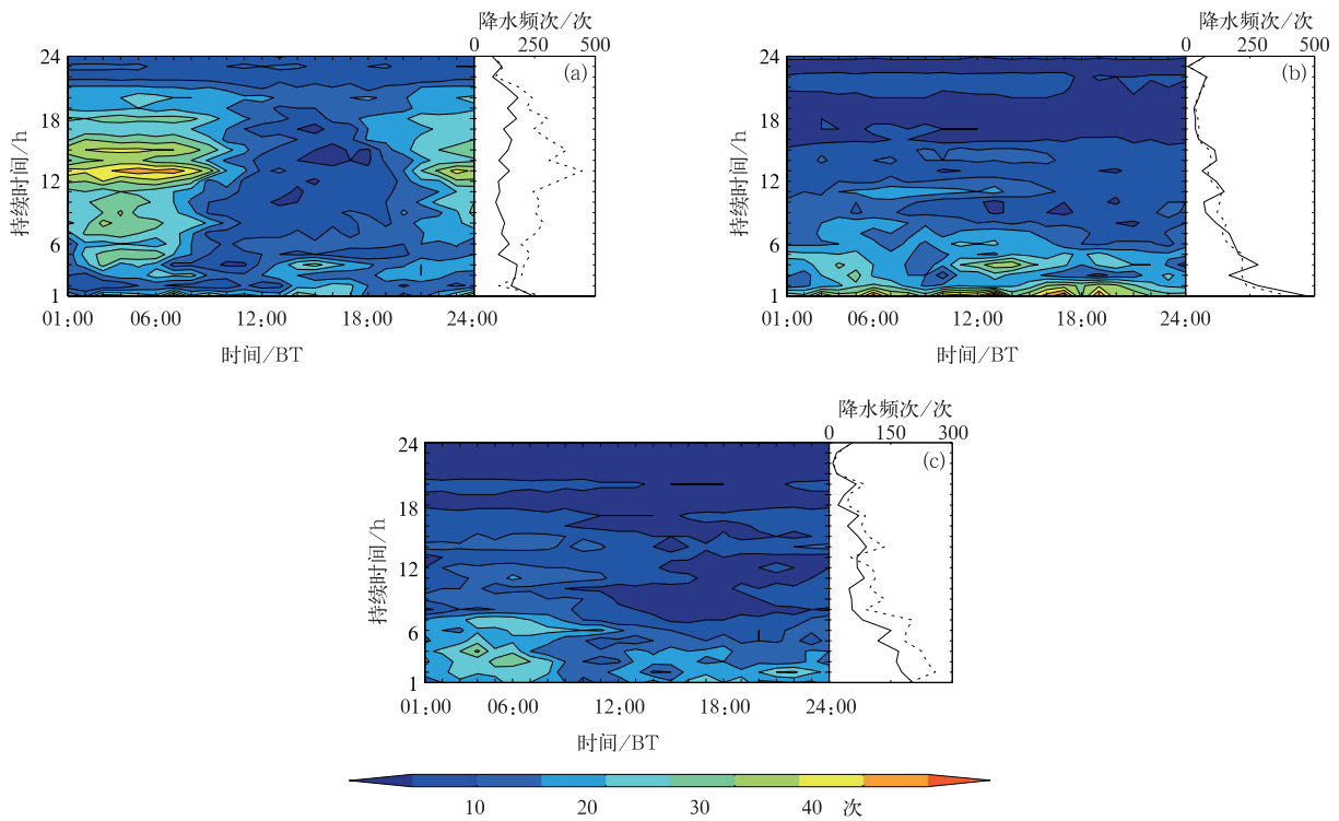
图 4 (a)山顶站、(b)山腰站、(c)坝区站不同持续时间的降水频次变化 Fig. 4 Rainfall frequency for different durations from the three stations at (a) the hilltop, (b) the hillside, and (c) the dam of Cangshan Mountain
