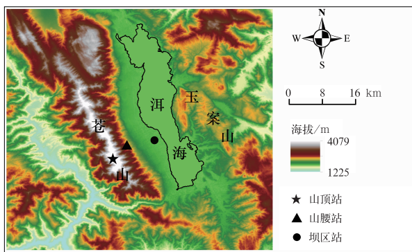
图 1 山顶站、山腰站和坝区站分布 Fig. 1 Distribution of the three stations at the hilltop, the hillside and the dam of Cangshan Mountain
