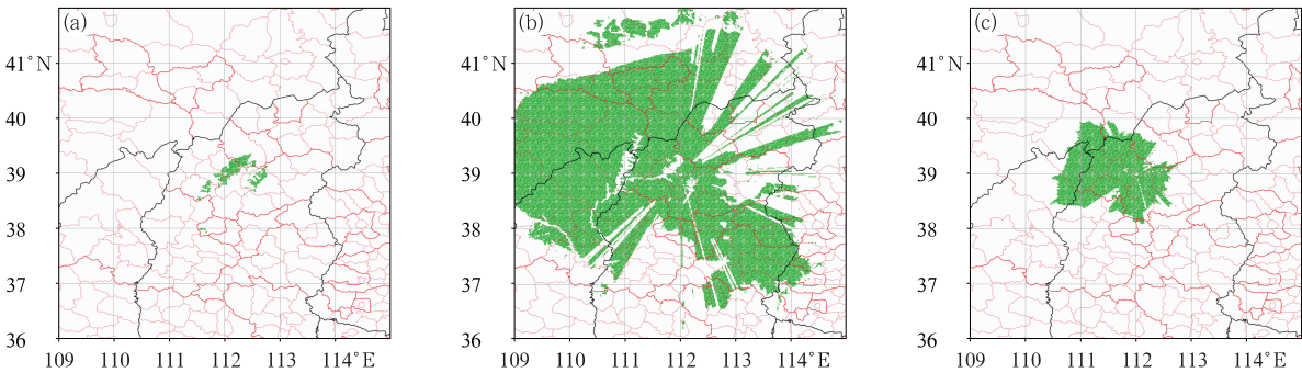
图 5 五寨雷达仰角下沿为(a) -0.1^{\circ} ,(b) -0.9^{\circ} ,(c) -1.3^{\circ} 时 1 km 高度覆盖范围 Fig. 5 The 1 km altitude coverage of Wuzhai Radar with elevation angle bottom edge at (a) -0.1^{\circ} , (b) -0.9^{\circ} , and (c) -1.3^{\circ}
