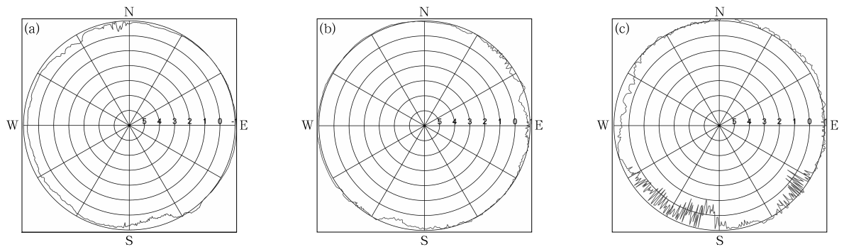
图 3 (a)固原,(b)五寨,(c)神农架 3 部雷达的遮蔽角 Fig. 3 The radar masking angle of the three radars in (a) Guyuan, (b) Wuzhai and (c) Shennongjia
