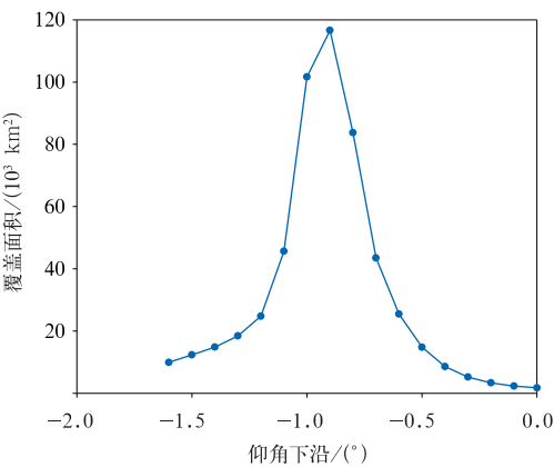
图 4 五寨雷达不同仰角下沿 1 km 高度覆盖面积 Fig. 4 Coverage area of Wuzhai Radar at 1 km height at different elevations
