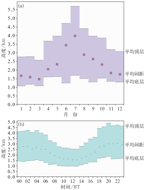
图 6 2016 年 1 月 1 日至 2020 年 12 月 31 日 (a)月份和(b)小时的多层云云底间距 Fig. 6 (a) Monthly and (b) hourly cloud-base height difference between the lowest layer cloud and the highest layer cloud in the case of multi-layer cloud from 1 January 2016 to 31 December 2020
