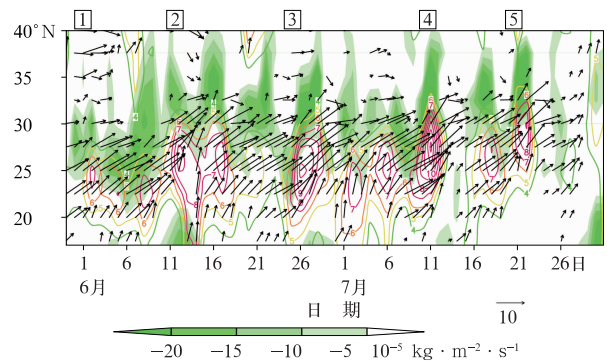
图 5 2020 年梅雨期 110^{\circ}\sim 122.5^{\circ}\text{E} 平均的 850 hPa 经向风(等值线, >1\text{ m}\cdot\text{s}^{-1} )和矢量风(箭头,单位: \text{m}\cdot\text{s}^{-1} )及整层水汽通量散度(填色)的时间-纬度剖面 (图片上方的数字表示 5 次低层南风大值中心的建立加强过程) Fig. 5 Time-latitude cross-section of the 850 hPa meridional wind (contours, >1\text{ m}\cdot\text{s}^{-1} ) and southwesterly wind (vectors, unit: \text{m}\cdot\text{s}^{-1} ) along 110^{\circ}\sim 122.5^{\circ}\text{E} , and divergence of the vertically integrated water vapor transport from surface to 300 hPa (colored) in the Meiyu season of 2020 (The numbers at the top of figure indicate five establishment and strengthening processes of the low-level southerly centers)
