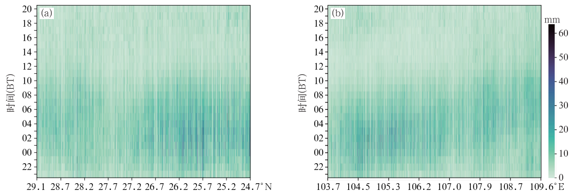
图8 2010—2023年汛期贵州暴雨小时降水量的(a)纬度-时间演变和(b)经度-时间演变 Fig. 8 (a) Latitude-time and (b) longitude-time evolutions of hourly precipitation of rainstorm in Guizhou Province during the flood season from 2010 to 2023
