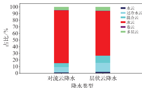
图 6 对流云和层状云降水的不同云类型占比 Fig. 6 Proportion of different cloud types for convective and stratiform precipitations
