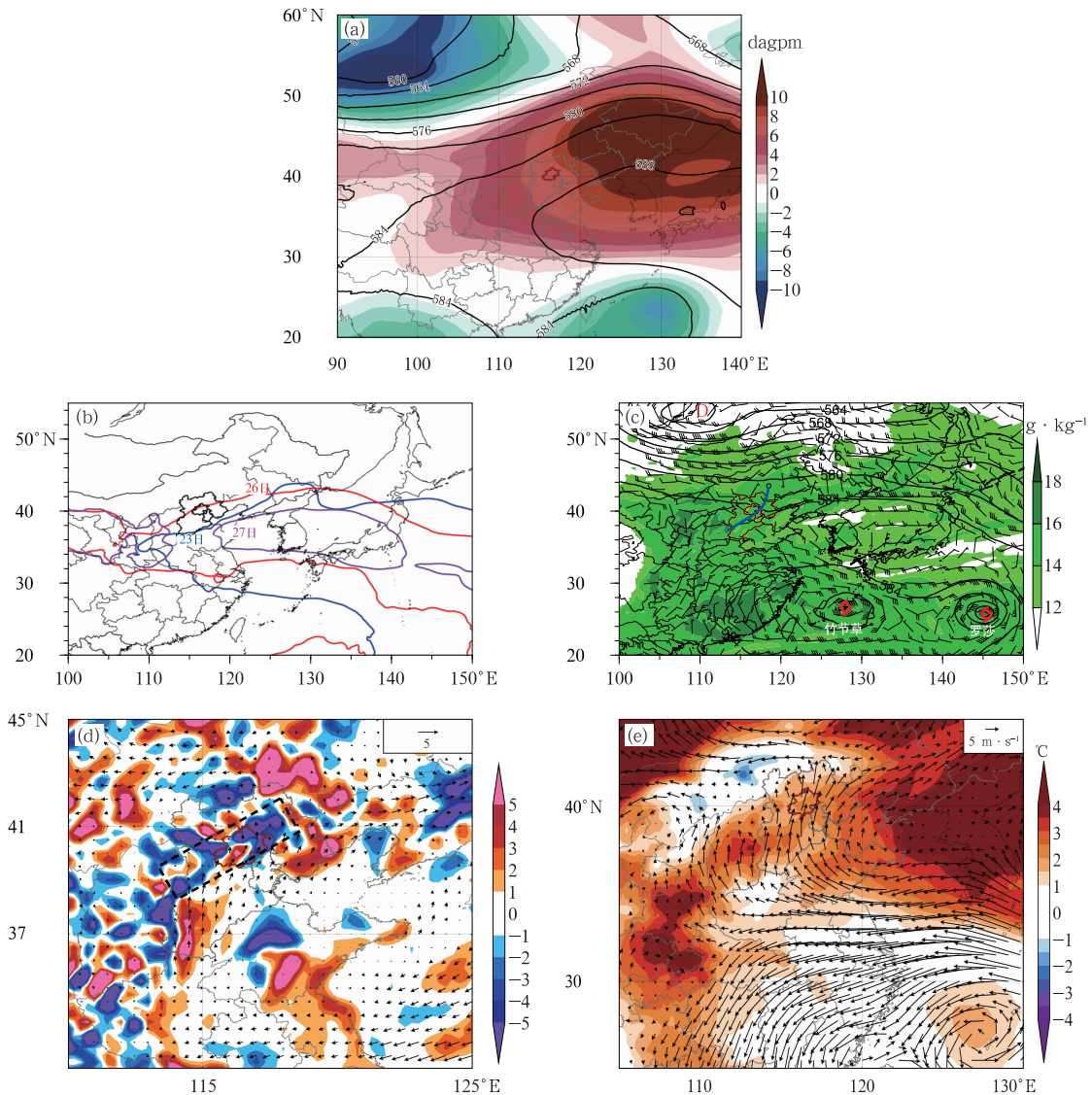
图 10 2025 年 7 月(a)23 日 500 hPa 位势高度(等值线,单位:dagpm)及其距平(填色),(b)副高 588 dagpm 线位置变化,(c)28 日 08:00 500 hPa 位势高度(等值线,单位:dagpm)、700 hPa 风场(风羽)和比湿(填色),(d)26 日 925 hPa 水汽通量散度(填色,单位: 10^{-7} \text{ g} \cdot \text{hPa}^{-1} \cdot \text{cm}^{-2} \cdot \text{s}^{-1} )和水汽通量距平(箭矢,单位: \text{g} \cdot \text{hPa}^{-1} \cdot \text{cm}^{-1} \cdot \text{s}^{-1} ),(e)26 日 850 hPa 温度距平(填色)和风场距平(箭矢) Fig. 10 (a) Geopotential height (contour, unit: dagpm) and its anomaly (colored) at 500 hPa on 23 July, (b) variation in the 588 dagpm contour position of the subtropical high from 23 to 27 July, (c) geopotential height (contour, unit: dagpm) at 500 hPa and wind field (barb) and specific humidity (colored) at 700 hPa at 08:00 BT 28 July, (d) water vapor flux divergence (colored, unit: 10^{-7} \text{ g} \cdot \text{hPa}^{-1} \cdot \text{cm}^{-2} \cdot \text{s}^{-1} ) and water vapor flux anomaly (arrow, unit: \text{g} \cdot \text{hPa}^{-1} \cdot \text{cm}^{-1} \cdot \text{s}^{-1} ) at 925 hPa, and (e) temperature anomaly (colored) and wind field anomaly (arrow) at 850 hPa on 26 July 2025
