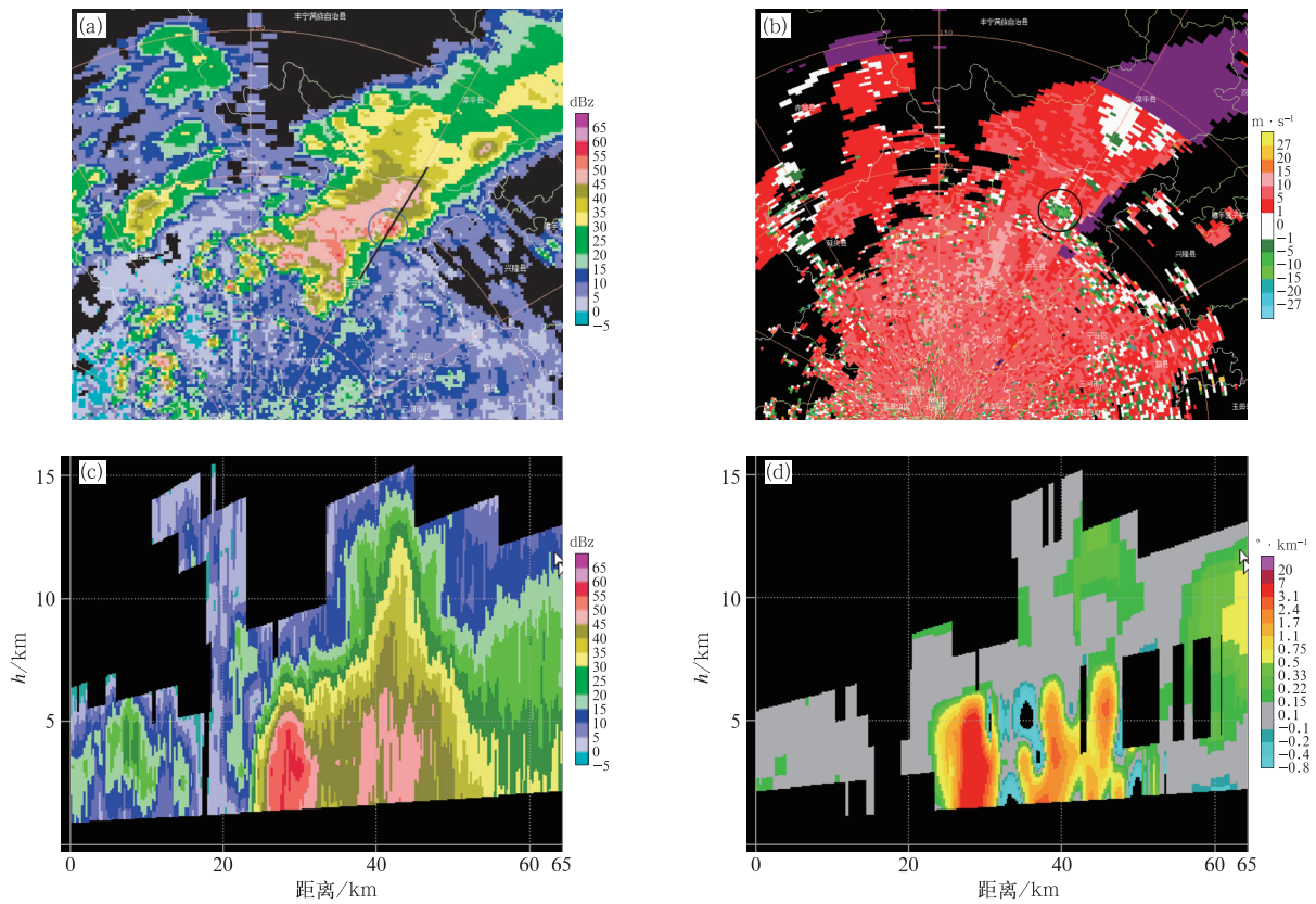
Fig. 6 Evolution of radar composite reflectivity factor from 26 to 27 July 2025
