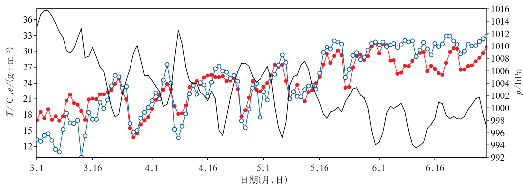
图 3 2023 年 3—6 月广州逐日平均气压(黑线)、温度(红线)、绝对湿度(蓝线)的变化 Fig. 3 Variations of daily average pressure (black line), temperature (red line), and absolute humidity (blue line) in Guangzhou from March to June 2023
